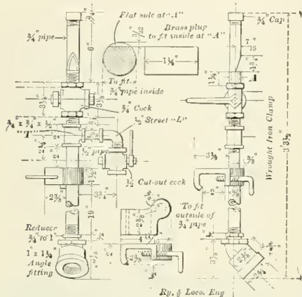
"BACK-UP" HOSE AND CONNECTIONS USED ON LEHIGH VALLEY R. R.
